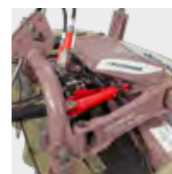
Hydraulic lateral displacement system
